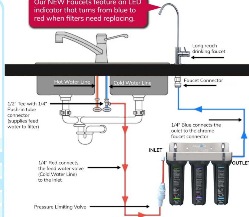
Triple Undersink w/ Sediment, Fluoride and Aragon
